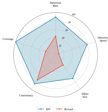
Figure 4 DT diagnostic profile. IDT (blue) outperforms reward (red) across all five dimensions: detection rate, speed, effect size, consistency, and coverage.
